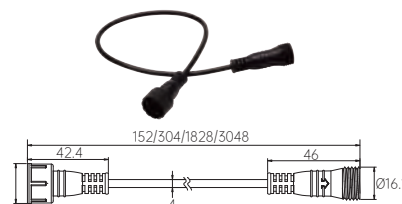
Joiner灯带连接线
